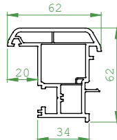
Lap Joint Profile Code: 41100-09000
