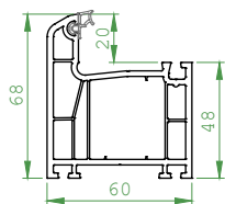
Super Frame Profile Code: 41100-92000
