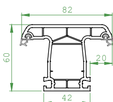
Mullion Profile Code: 41100-93000
