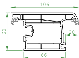
Out Opening Door Sash Profile Code: 41100-98000
