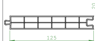
Panel Profile (20x125 mm) Code: 40102-04000
