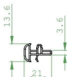
Coupling Profile Code: 40106-01000
