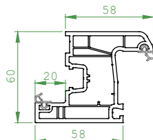
Sash Profile Code: 41100-95000
