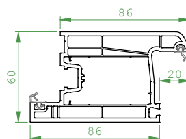
Door Sash Profile Code: 41100-97000
